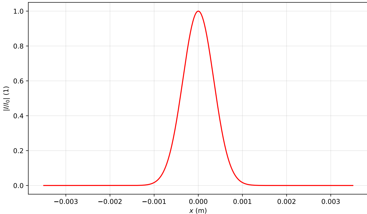
Intensity profile I(x, y = 0, z = 0.000)/I_0 , P_{in}=4.5P_{cr} , artificial time
